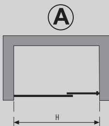
A Hoja fija + hoja corredera + kit Fixed glass + slide glass + kit Lame fixe + lame mobile + kit
