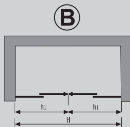
B Dos hojas fijas + dos hojas correderas Two fixed glasses + two slide glasses Deux lames fixes + deux lames mobiles
