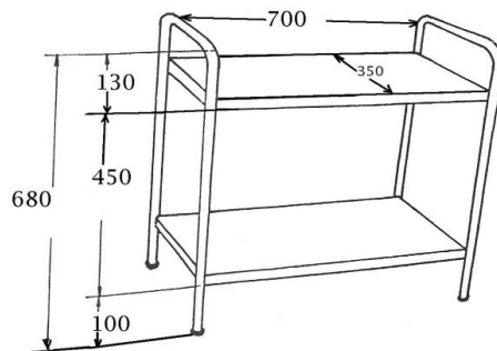
CARUCIOR 2.3 680 X 700 X 350
