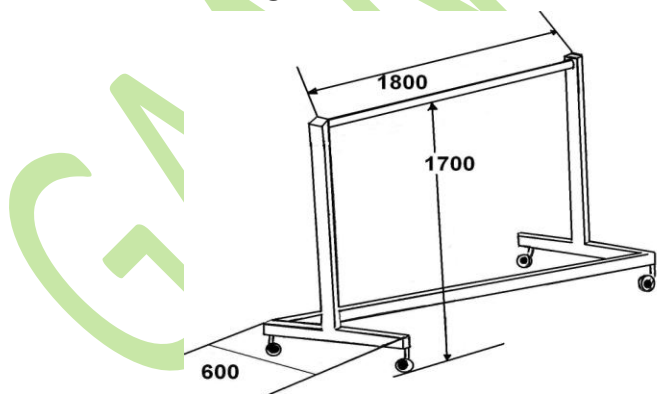
STENDER BAZA "Z"
